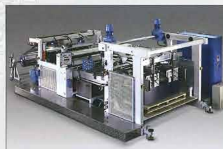
Stacking on elevating platform
