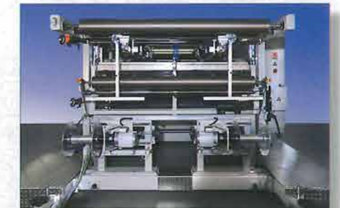
Option: edge trimming tab winding
